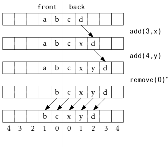
Figure 2.4: A sequence of \text{add}(i, x) and \text{remove}(i) operations on a DualArray-Deque. Arrows denote elements being copied. Operations that result in a rebalancing by \text{balance}() are marked with an asterisk.
