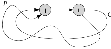
Figure 12.6: The depth-first-search algorithm can be used to detect cycles in G . The node j is coloured grey while i is still grey. This implies that there is a path, P , from i to j in the depth-first-search tree, and the edge (j, i) implies that P is also a cycle.
