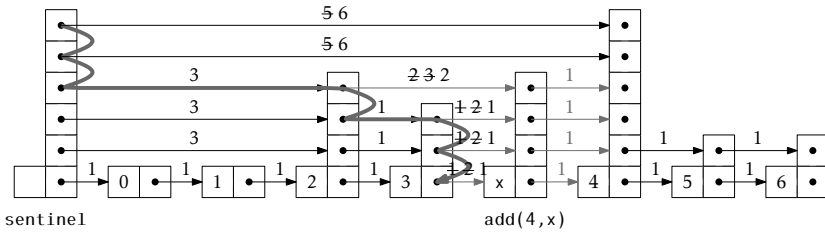
Figure 4.6: Adding an element to a SkiplistList.
