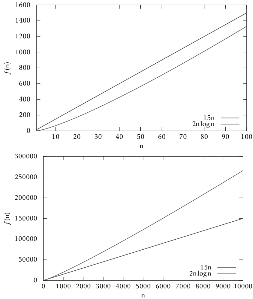
Figure 1.5: Plots of 15n versus 2n \log n .
