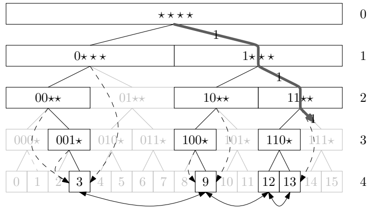
Figure 13.6: The search path for 14 (1110) ends at the node labelled 110* since there is no node labelled 111*.
