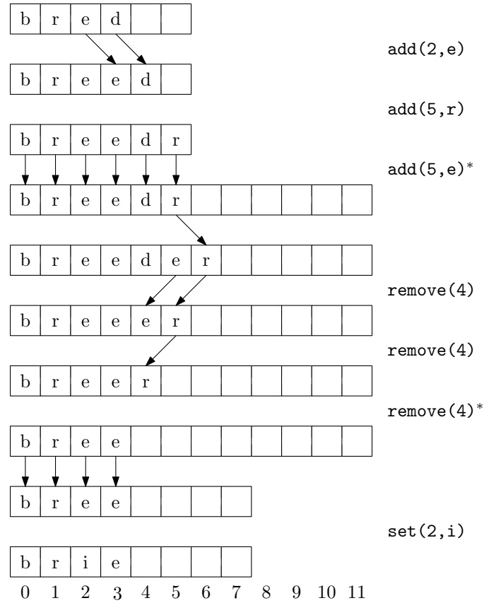
Figure 2.1: A sequence of \text{add}(i, x) and \text{remove}(i) operations on an ArrayStack . Arrows denote elements being copied. Operations that result in a call to resize() are marked with an asterisk.
