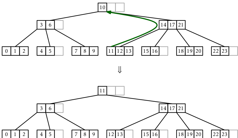
Figure 14.8: The \text{remove}(x) operation in a BTree. To remove the value x = 10 we replace it with the value x' = 11 and remove 11 from the leaf that contains it.
