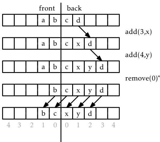
Figure 2.4: A sequence of \text{add}(i,x) and \text{remove}(i) operations on a DualArrayDeque. Arrows denote elements being copied. Operations that result in a rebalancing by \text{balance}() are marked with an asterisk.
