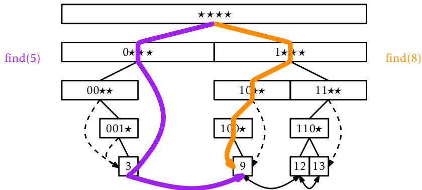
Figure 13.3: The paths followed by \text{find}(5) and \text{find}(8) .
