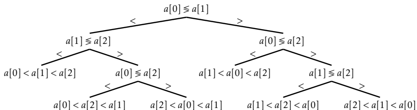
Figure 11.5: A comparison tree for sorting an array a[0], a[1], a[2] of length n \leftarrow 3 .
