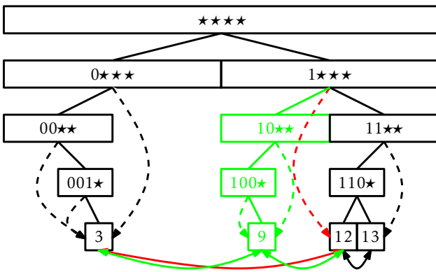
Figure 13.5: Removing the value 9 from the BinaryTrie in Figure 13.2.
