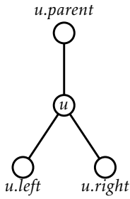
Figure 6.1: The parent, left child, and right child of the node u in a BinaryTree.
