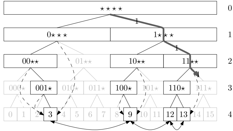
Figure 13.6: The search path for 14 (1110) ends at the node labelled 110* since there is no node labelled 111*.
