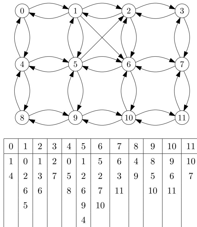
Figure 12.3: A graph and its adjacency lists
